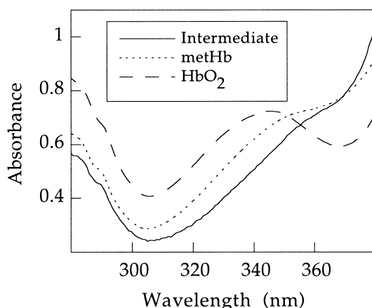
Fig. 4. Spectral changes in the range between 280 and 380 nm during the NO * -mediated oxidation of HbO 2 . The spectrum of the intermediate was obtained from a reaction of 13 μM HbO 2 with ca. 30 μM NO * in 0.1 M borate buffer at pH 9.5, 5°C.
